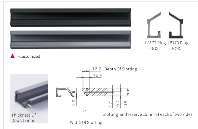
L8173 Material:Aluminium Alloy Color:MAB/MN/MBL C L H W / 3000 22 43
