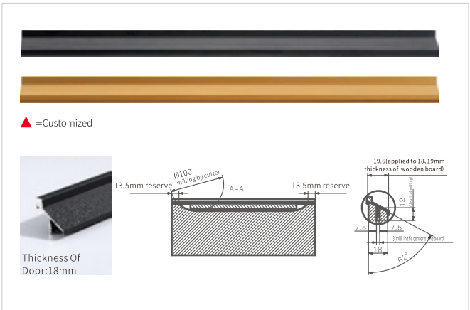
L8174 Material:Aluminium Alloy Color:Brass OX/BOX C L H W / 3000 10 22
